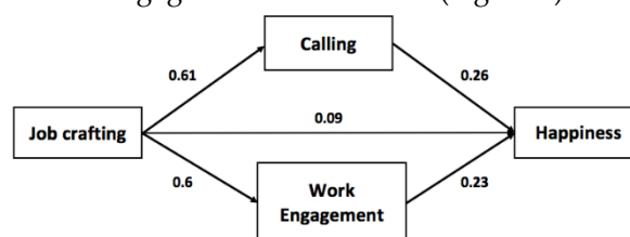
Figure 1. Mediation Model
